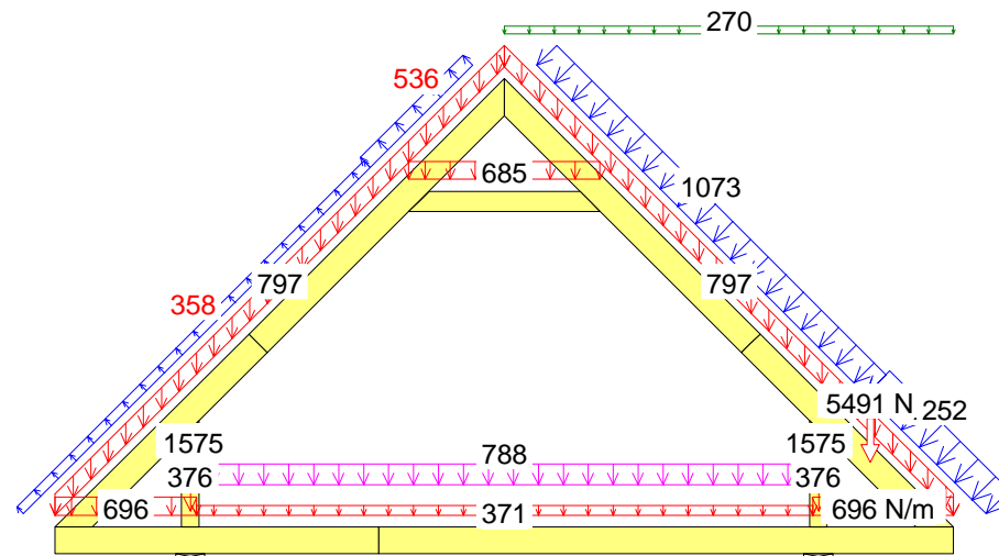
17 Kr 1.15*Stale+1.05*(OZ1+OZ2+OZ3)+0.75*ŚniegP(0L)+1.5*WiatrP
